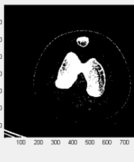
Thresholded Image
